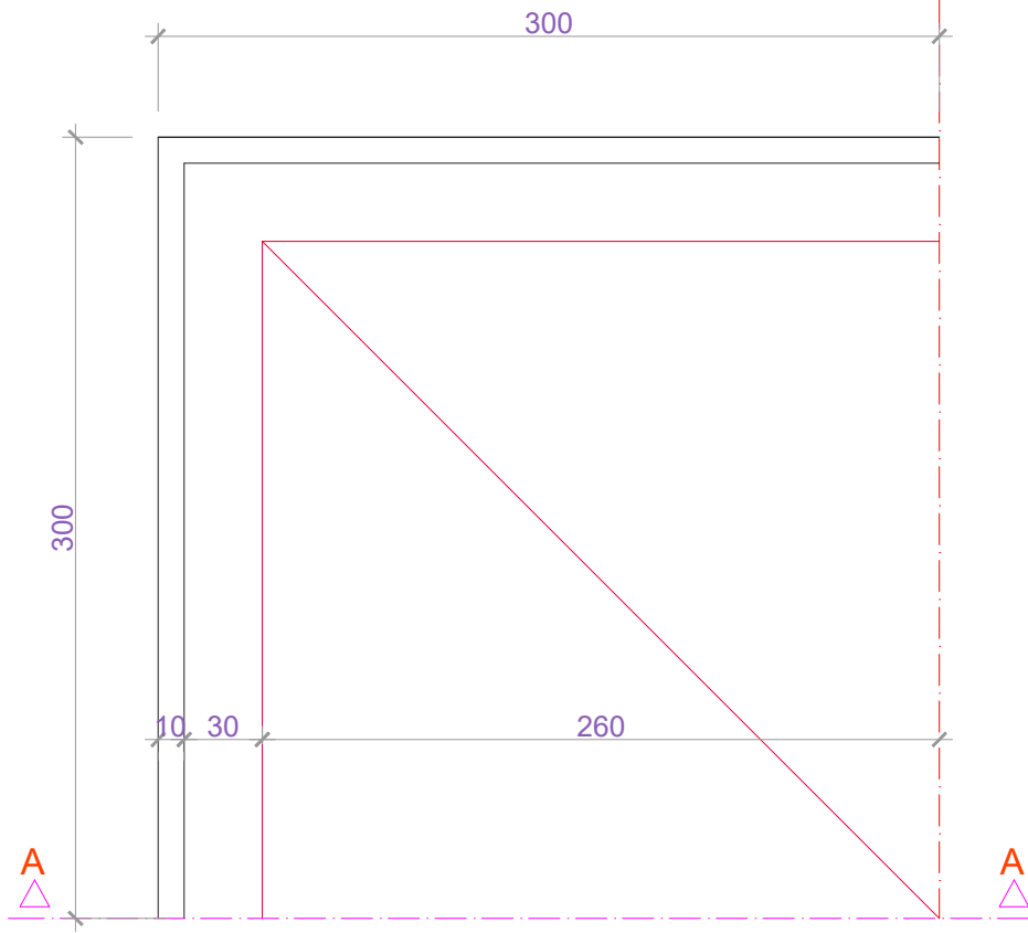
ÇATI PLANI
